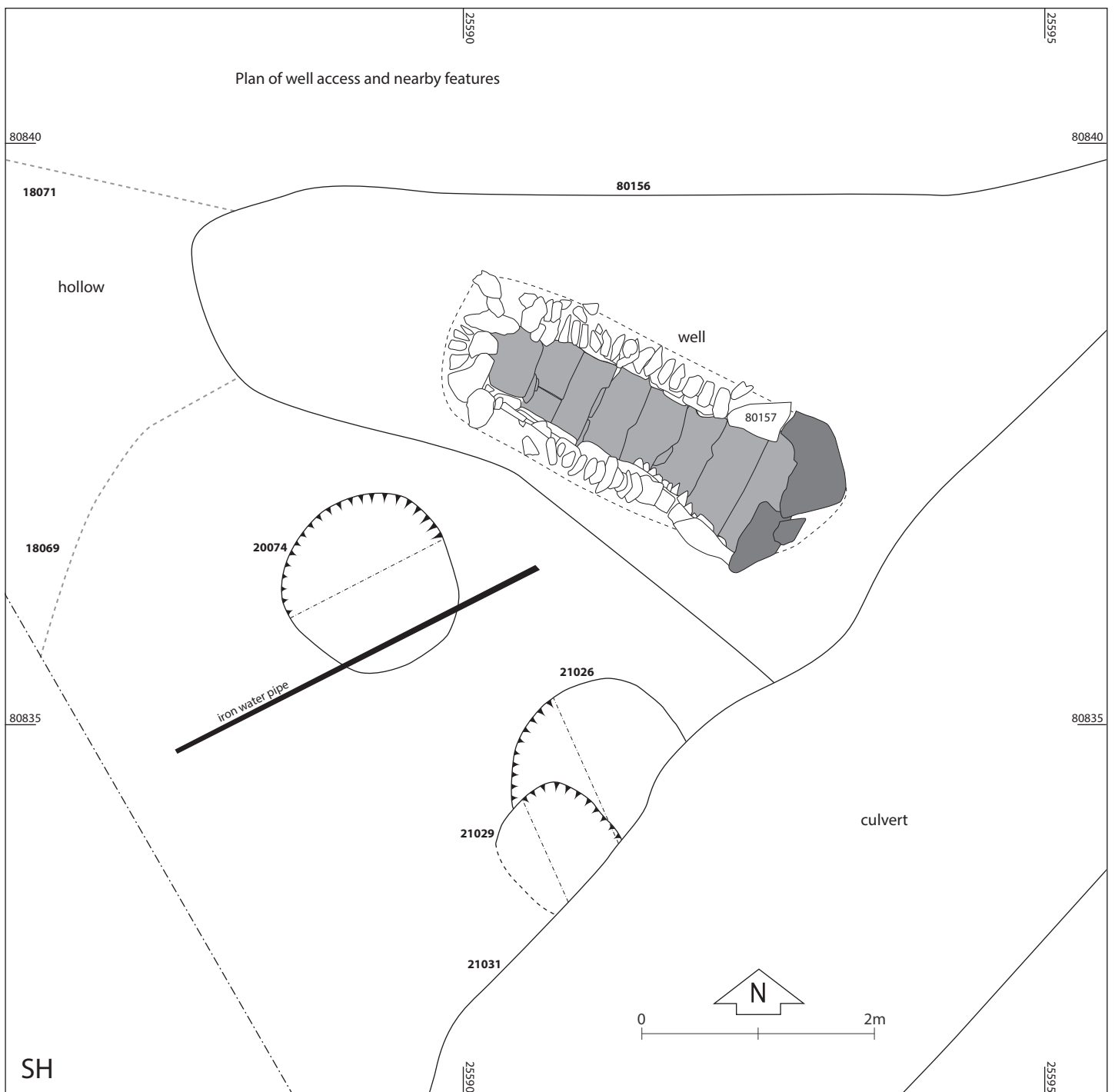
Figure 128. Plan and elevation of well PRN 31614
